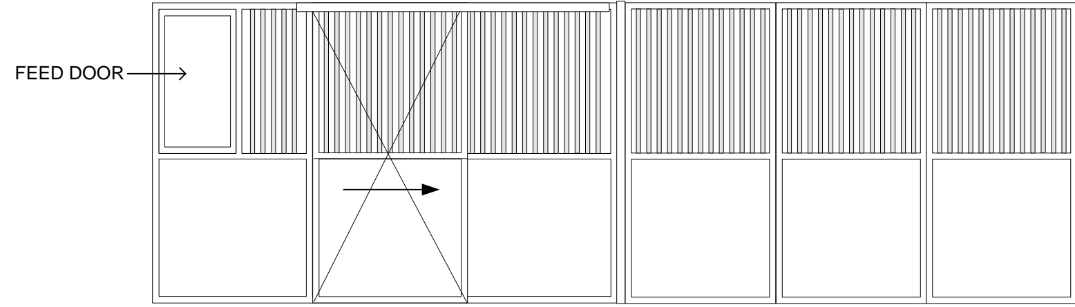
24' ESTATE STALL FRONT GALV. FRAME W/ 3/4" PTD PANELS
