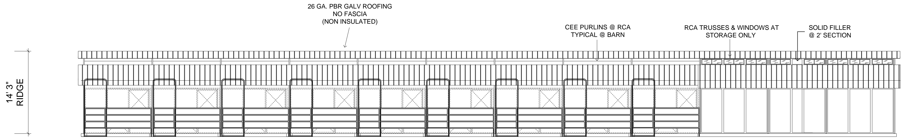
SIDE ELEVATION (WITH CORRAL RUNS)
