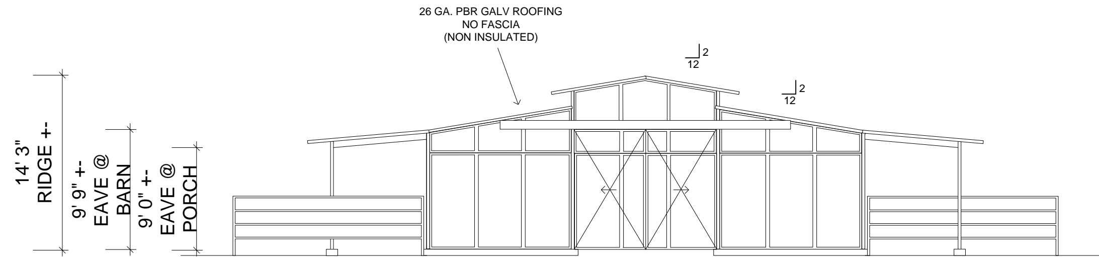
REAR ELEVATION
