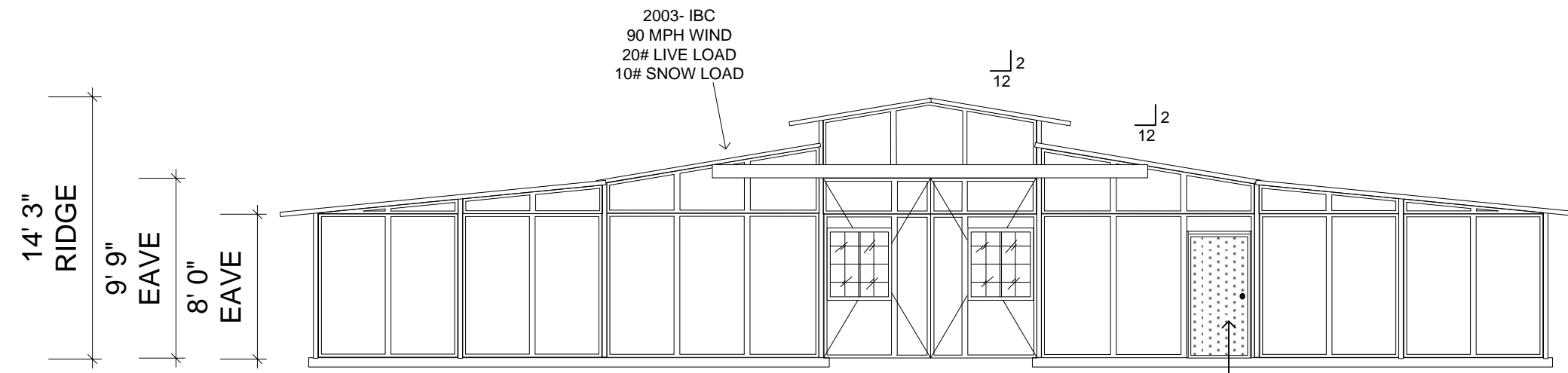
FRONT ELEVATION
