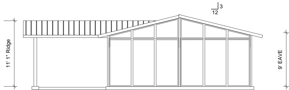
NORTH END ELEVATION
