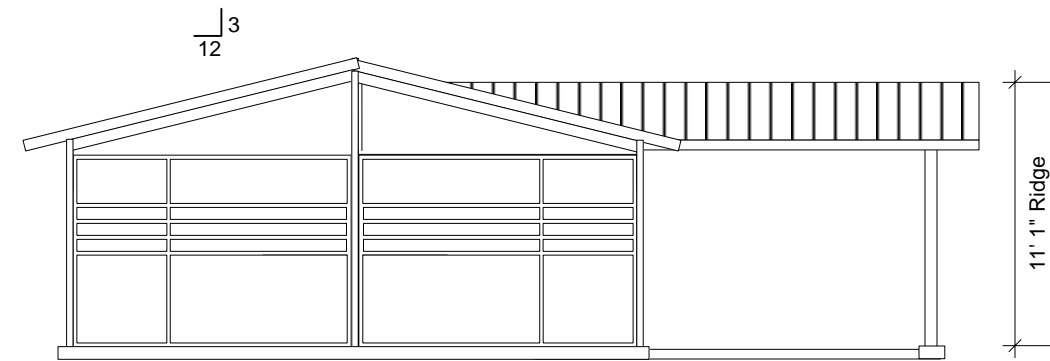
SOUTH END ELEVATION
